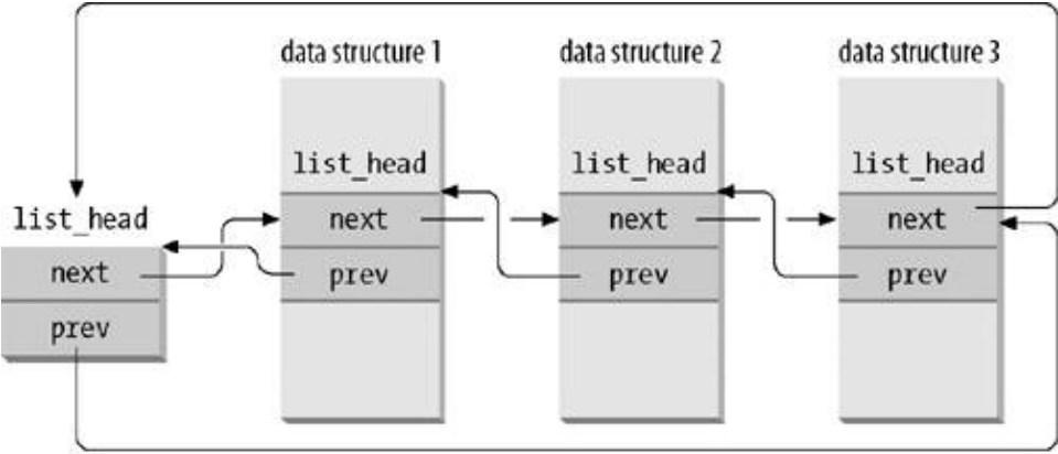
(a) a doubly linked listed with three elements
