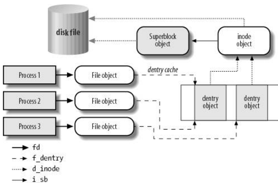
Figure 12-2. Interaction between processes and VFS objects
