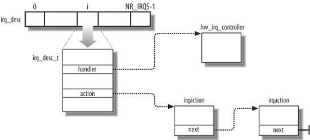
Figure 4-5. IRQ descriptors
