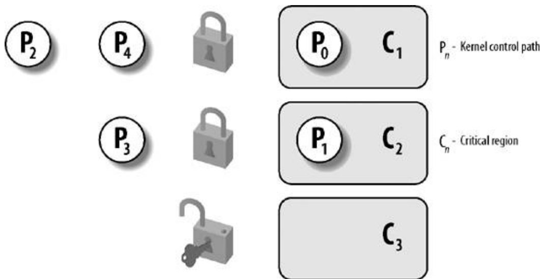
Figure 5-1. Protecting critical regions with several locks
